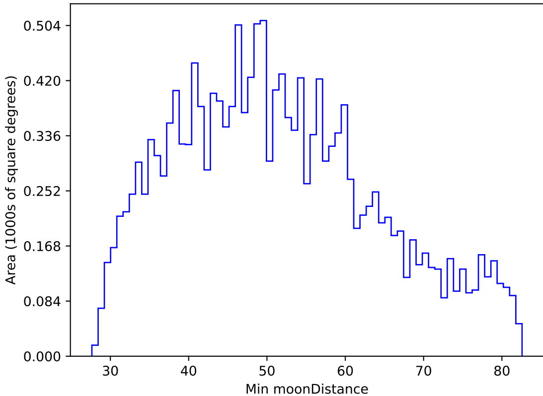
too_elab_r256_d2_ugrizy_v3.4_10yrs WFD u band: Min moonDistance
