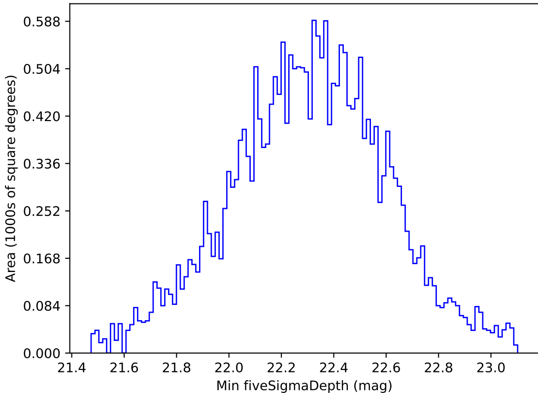
too_elab_r256_d2_ugrizy_v3.4_10yrs All sky u band: Min fiveSigmaDepth
