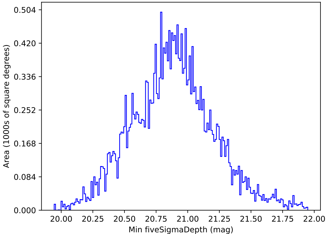
too_elab_r256_d2_ugrizy_v3.4_10yrs All sky all bands: Min fiveSigmaDepth
