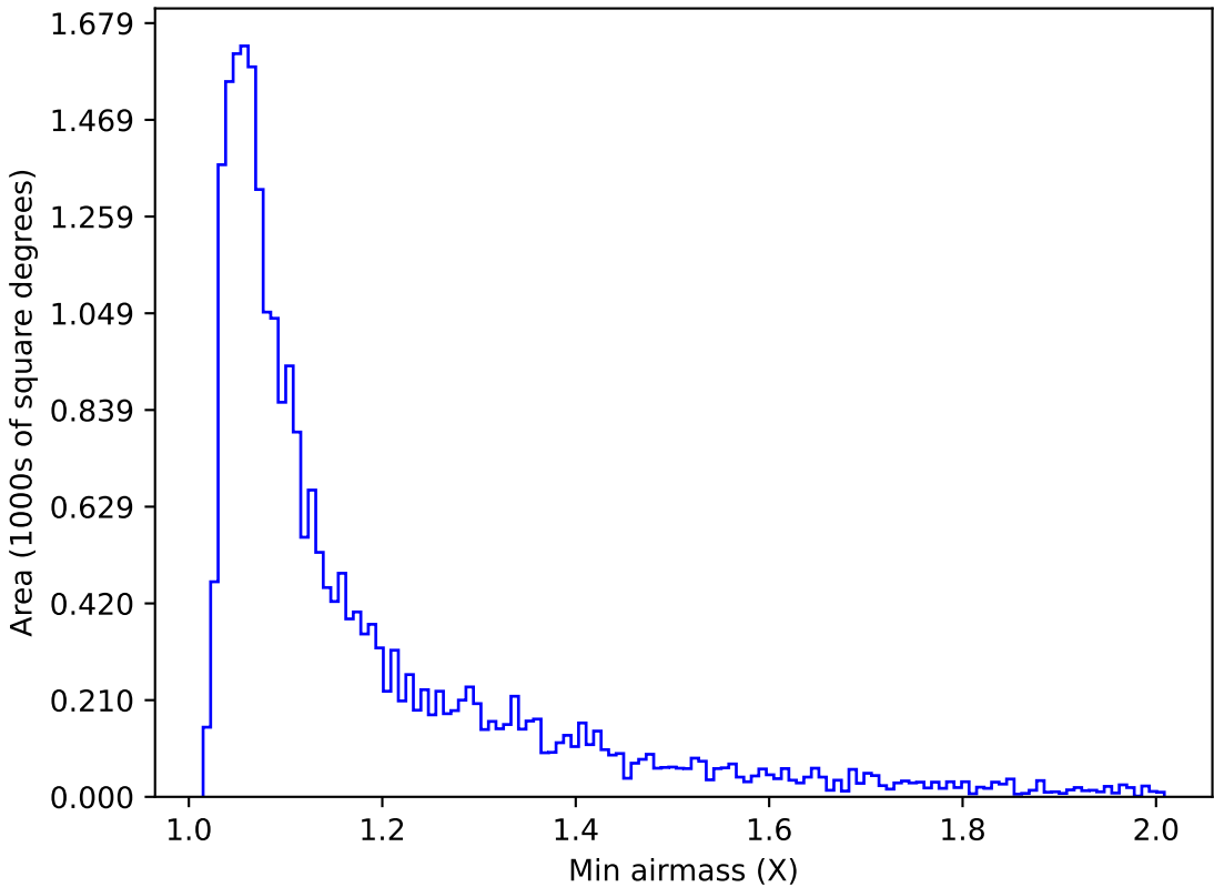
too_elab_r256_d2_ugrizy_v3.4_10yrs Yr 1 g band: Min airmass
