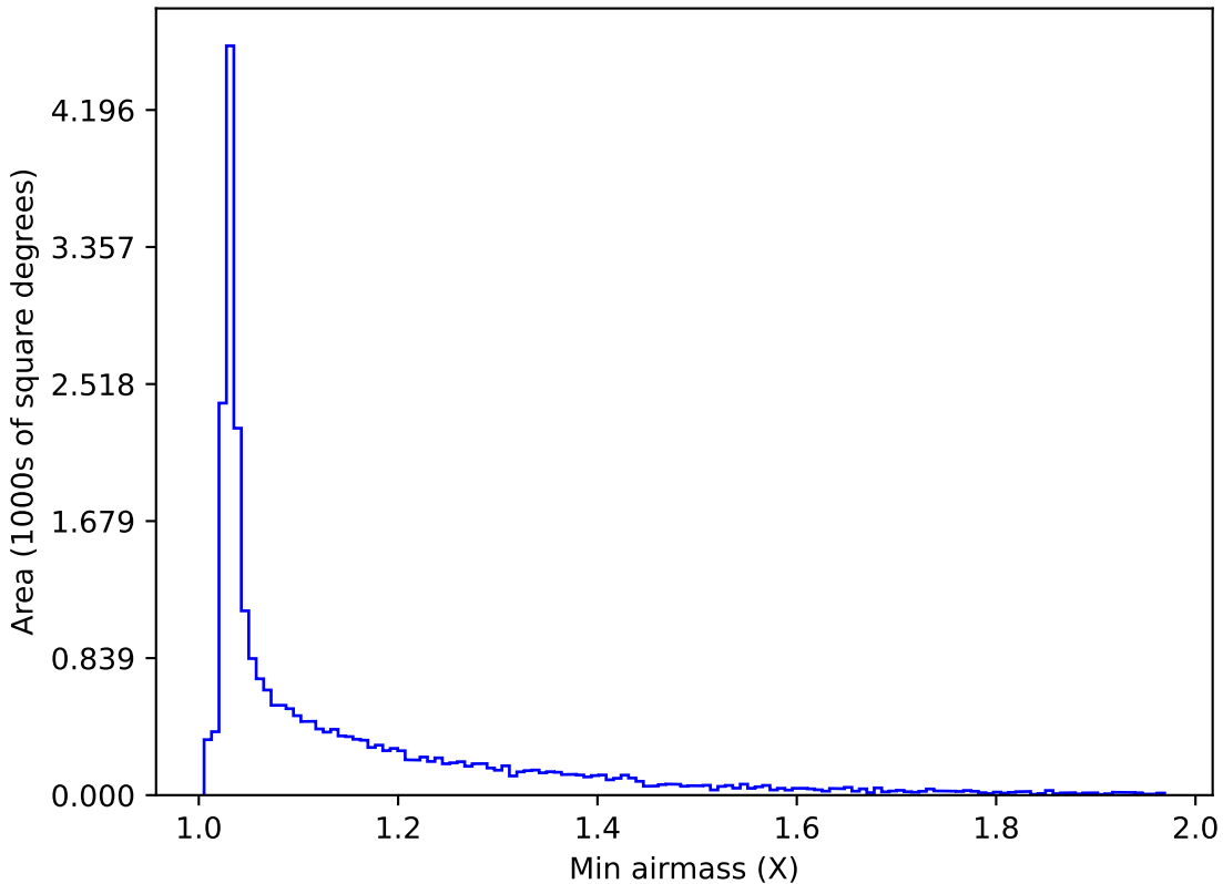
too_elab_r256_d2_ugrizy_v3.4_10yrs Yr 1 all bands: Min airmass
