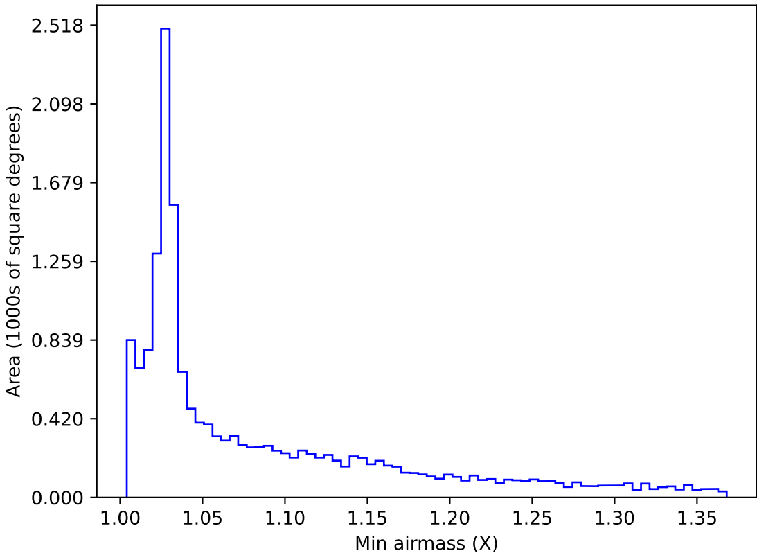
too_elab_r256_d2_ugrizy_v3.4_10yrs WFD z band: Min airmass
