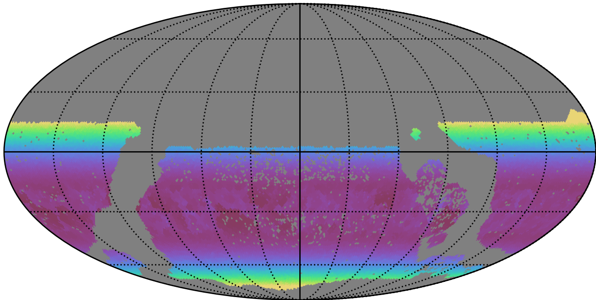
too_elab_r256_d2_ugrizy_v3.4_10yrs WFD u band: Min airmass
