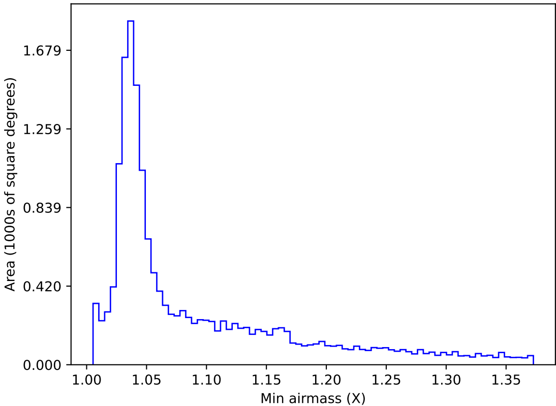
too_elab_r256_d2_ugrizy_v3.4_10yrs WFD u band: Min airmass
