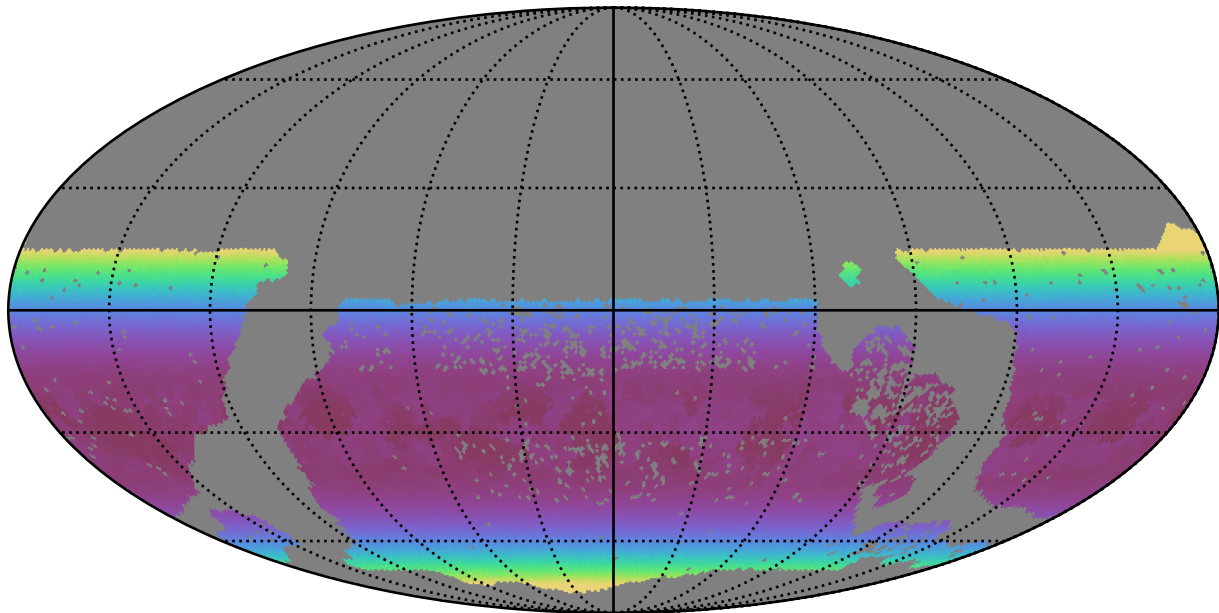
too_elab_r256_d2_ugrizy_v3.4_10yrs WFD r band: Min airmass
