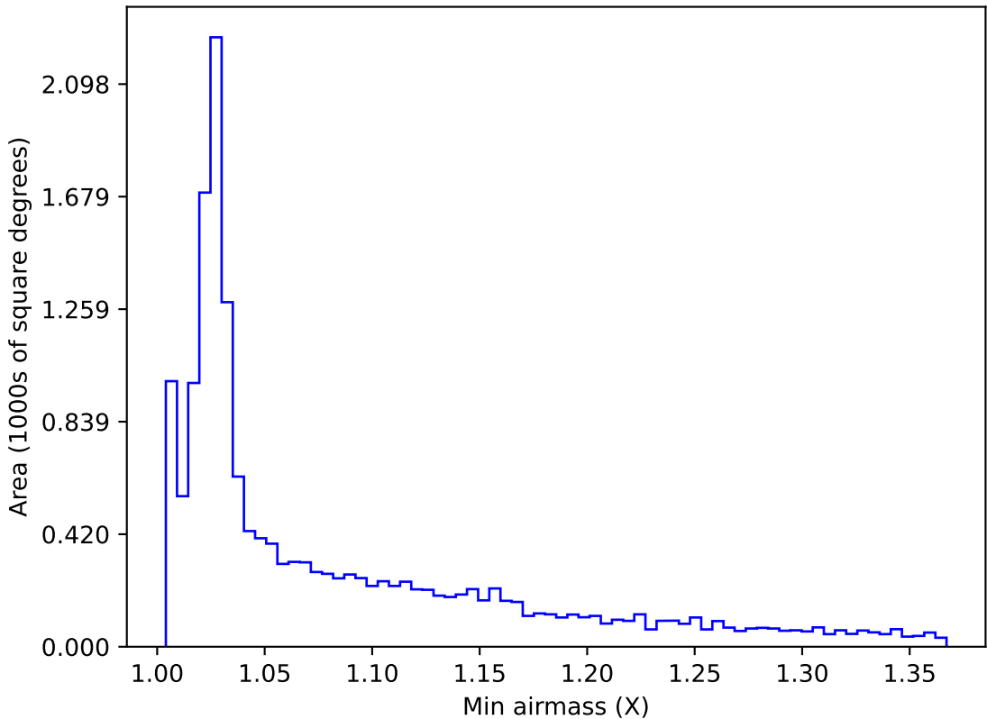
too_elab_r256_d2_ugrizy_v3.4_10yrs WFD r band: Min airmass
