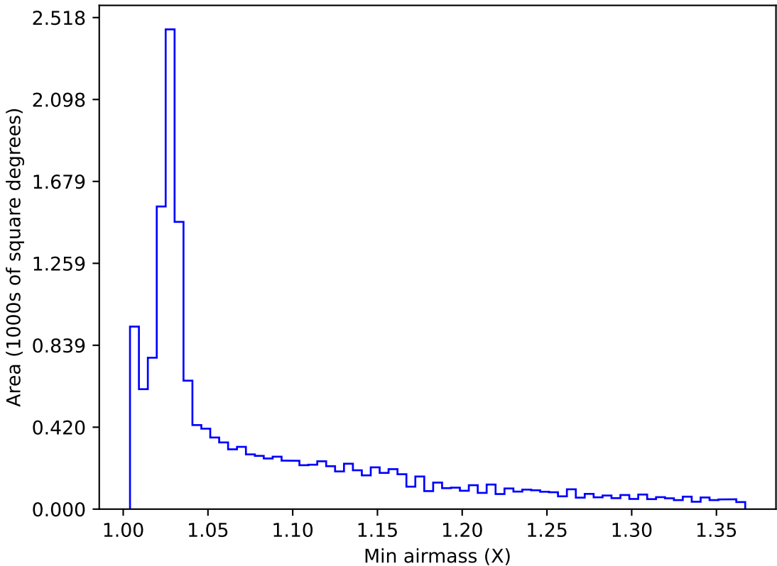
too_elab_r256_d2_ugrizy_v3.4_10yrs WFD i band: Min airmass
