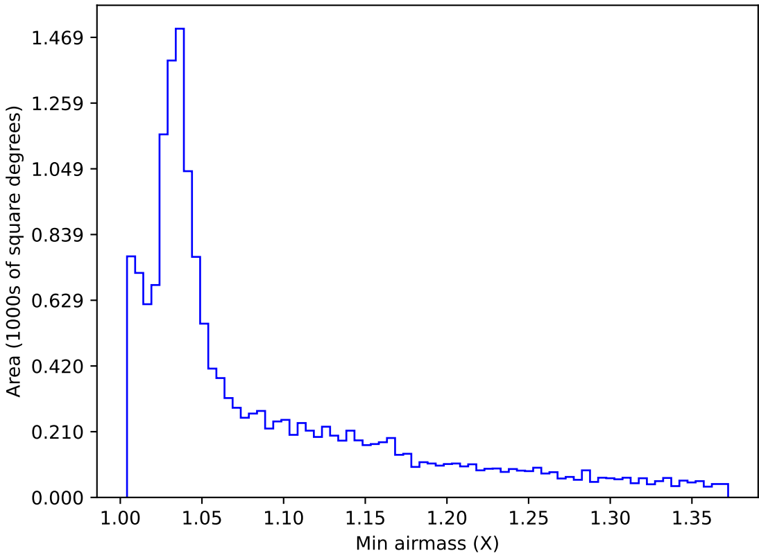
too_elab_r256_d2_ugrizy_v3.4_10yrs WFD g band: Min airmass
