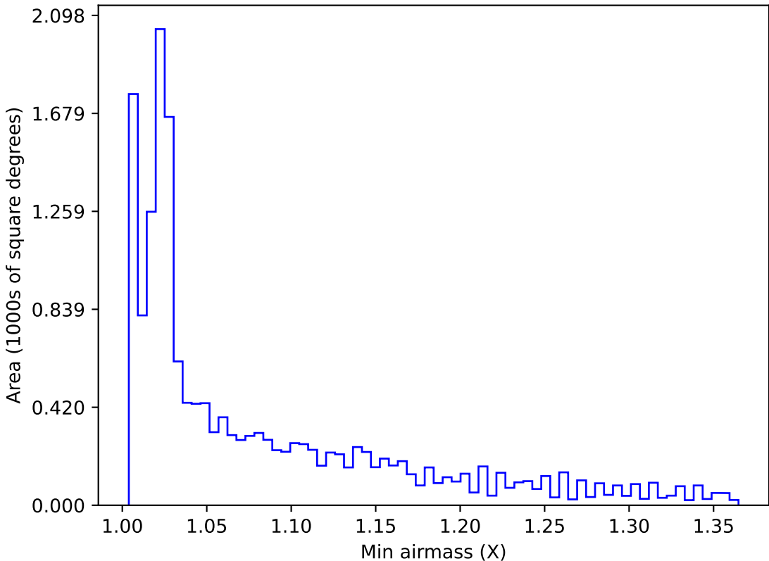
too_elab_r256_d2_ugrizy_v3.4_10yrs WFD all bands: Min airmass
