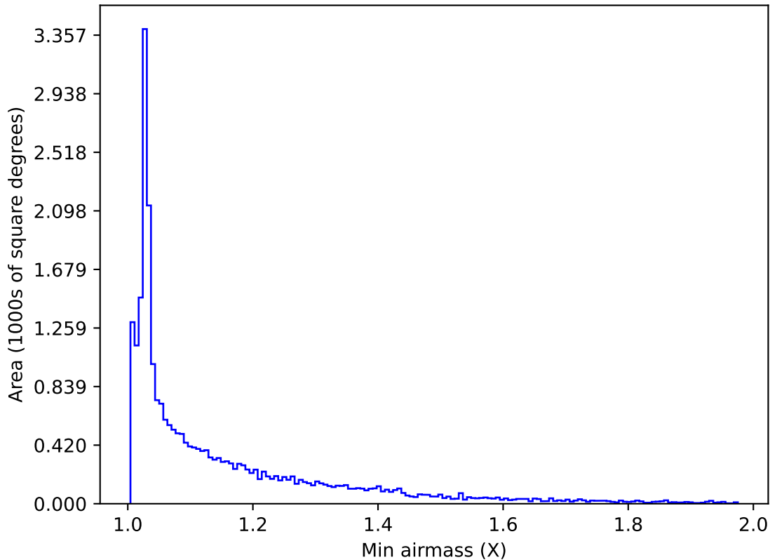
too_elab_r256_d2_ugrizy_v3.4_10yrs All sky z band: Min airmass
