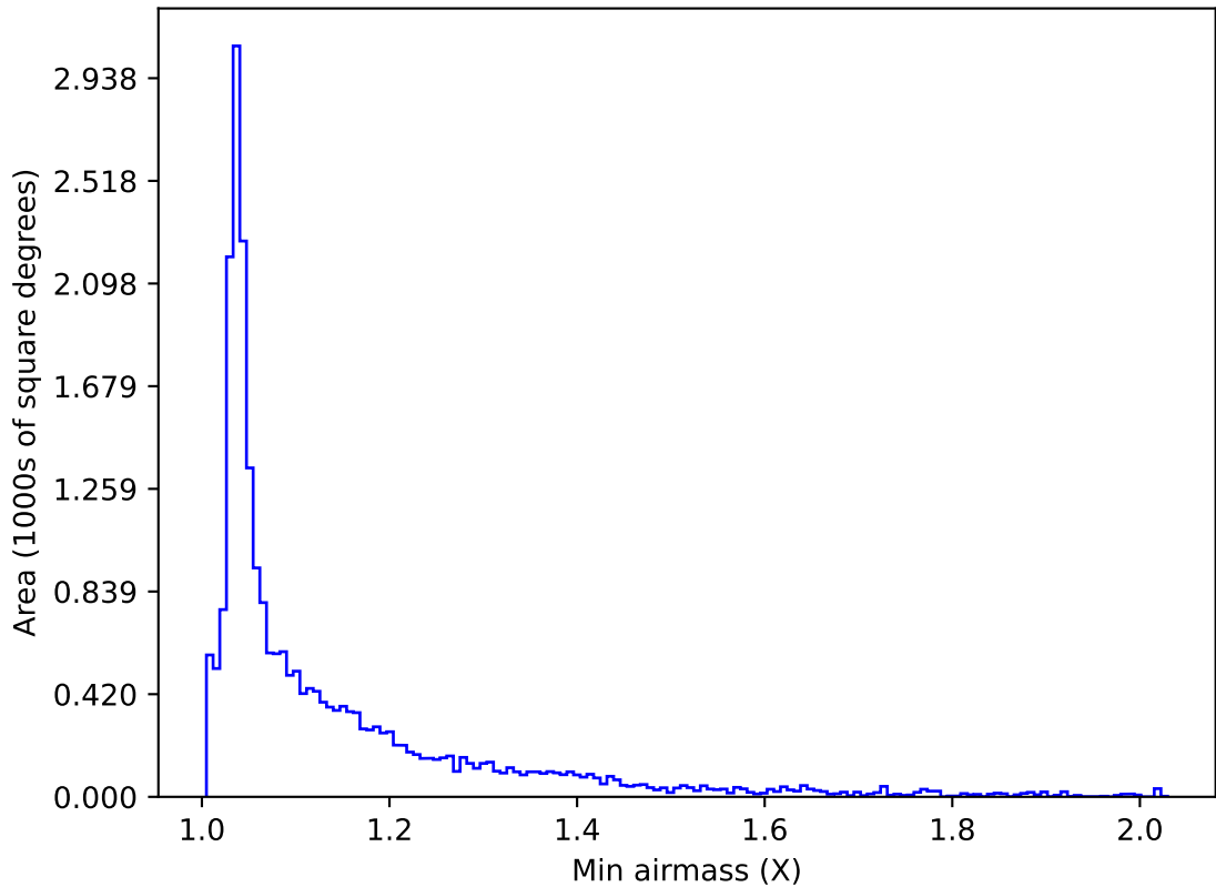
too_elab_r256_d2_ugrizy_v3.4_10yrs All sky u band: Min airmass
