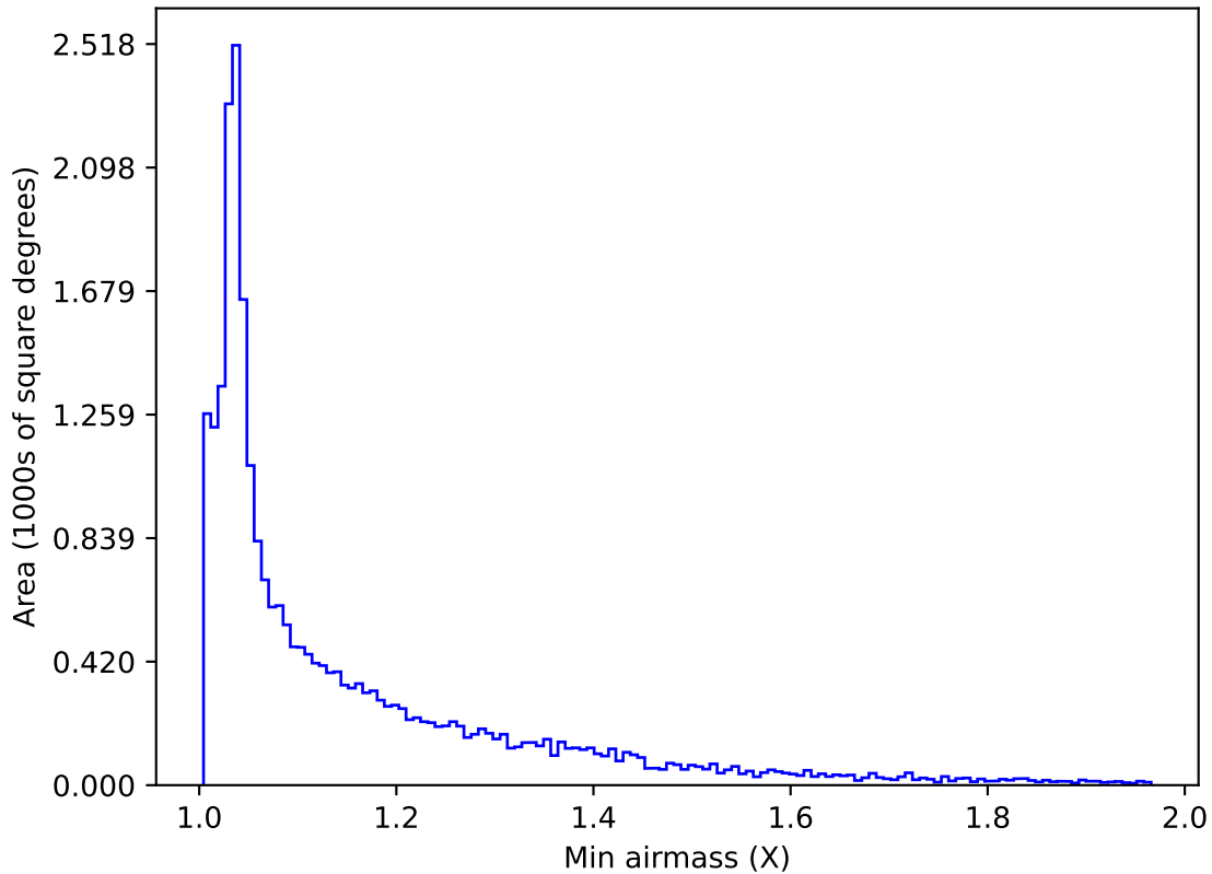
too_elab_r256_d2_ugrizy_v3.4_10yrs All sky g band: Min airmass
