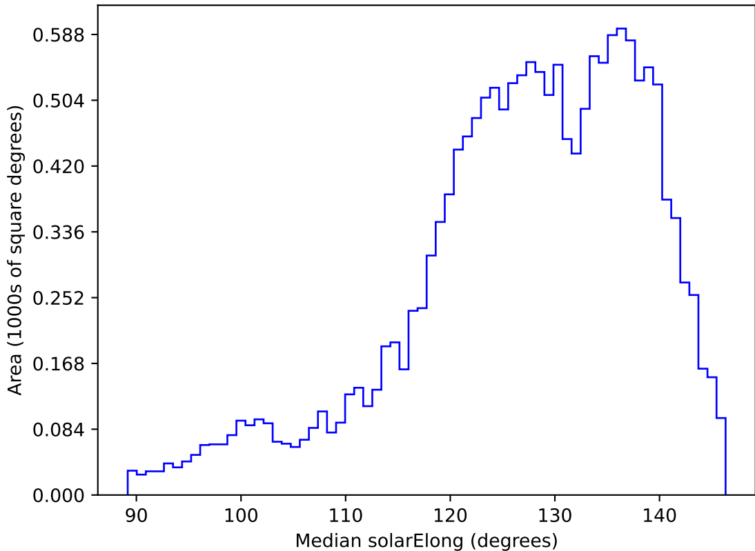
too_elab_r256_d2_ugrizy_v3.4_10yrs WFD z band: Median solarElong
