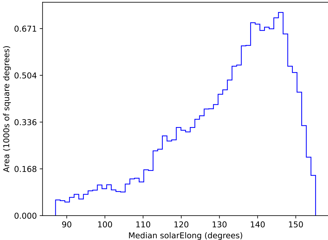
too_elab_r256_d2_ugrizy_v3.4_10yrs WFD u band: Median solarElong
