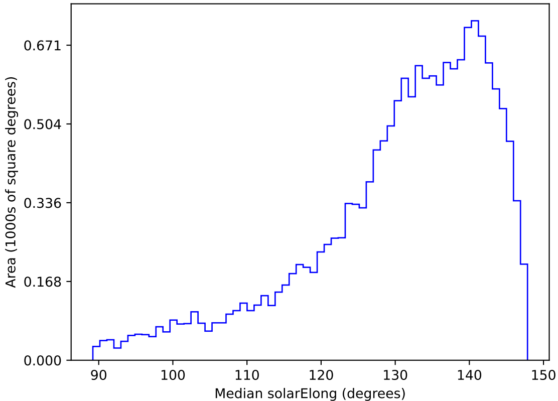
too_elab_r256_d2_ugrizy_v3.4_10yrs WFD r band: Median solarElong
