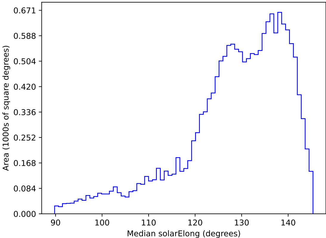
too_elab_r256_d2_ugrizy_v3.4_10yrs WFD i band: Median solarElong
