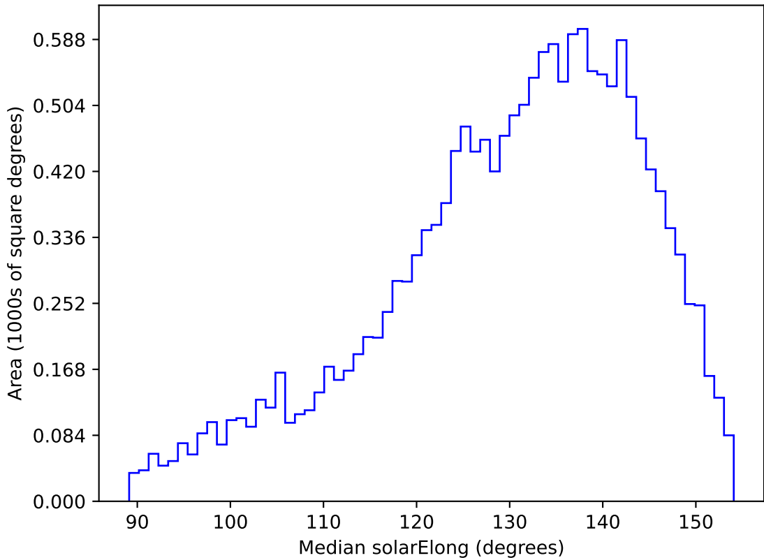
too_elab_r256_d2_ugrizy_v3.4_10yrs WFD g band: Median solarElong
