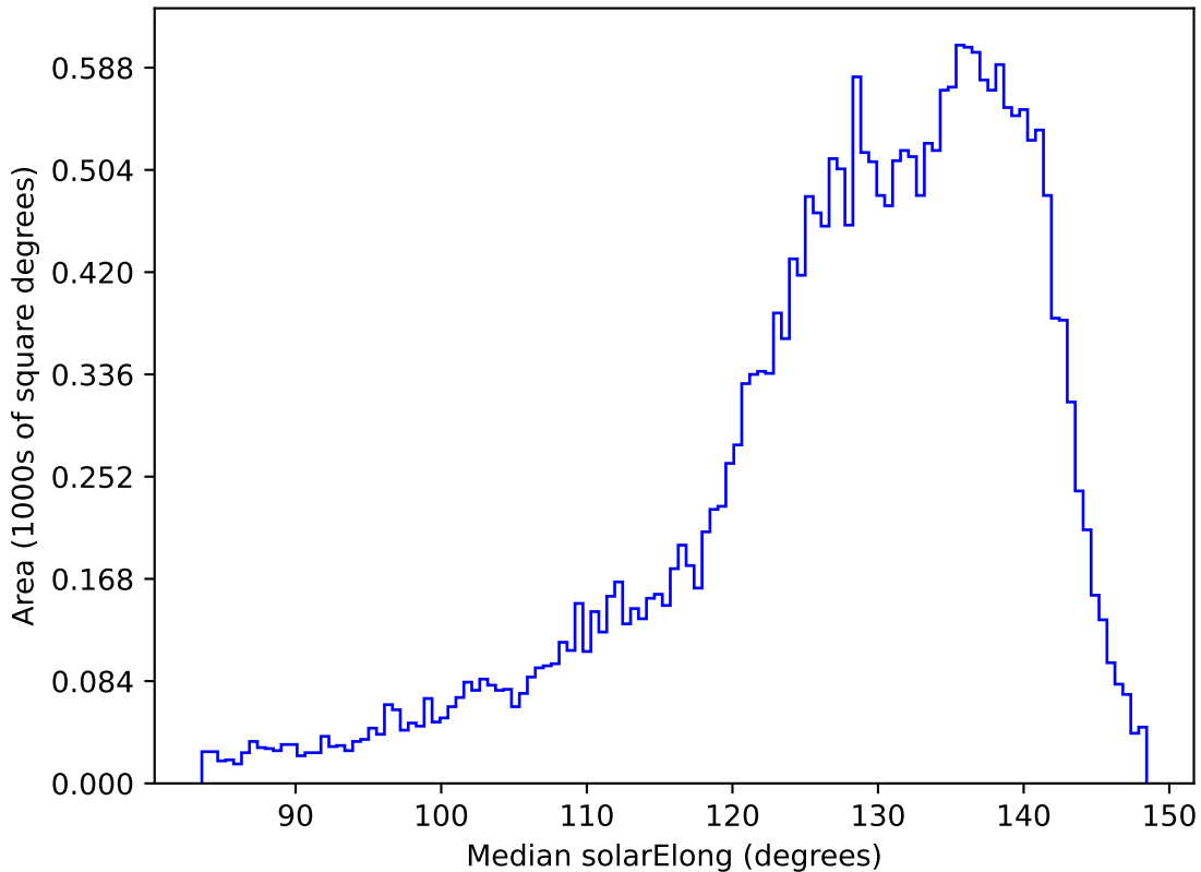
too_elab_r256_d2_ugrizy_v3.4_10yrs All sky i band: Median solarElong
