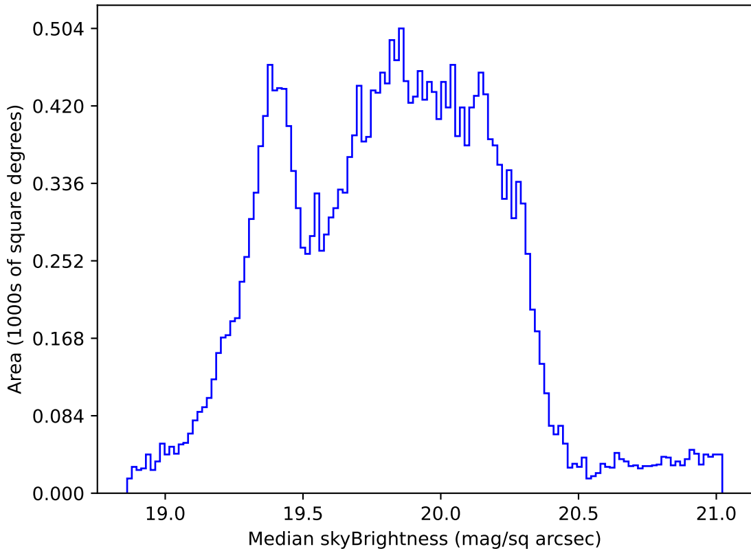
too_elab_r256_d2_ugrizy_v3.4_10yrs Yr 1 all bands: Median skyBrightness
