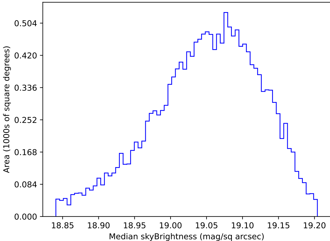
too_elab_r256_d2_ugrizy_v3.4_10yrs WFD z band: Median skyBrightness
