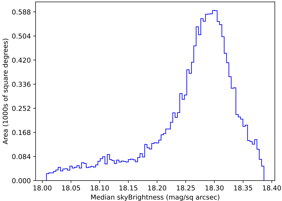
too_elab_r256_d2_ugrizy_v3.4_10yrs WFD y band: Median skyBrightness
