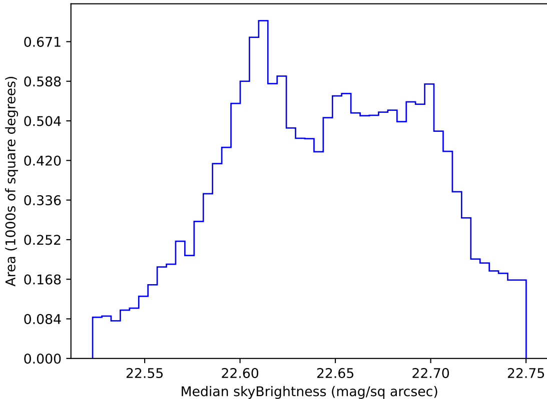
too_elab_r256_d2_ugrizy_v3.4_10yrs WFD u band: Median skyBrightness
