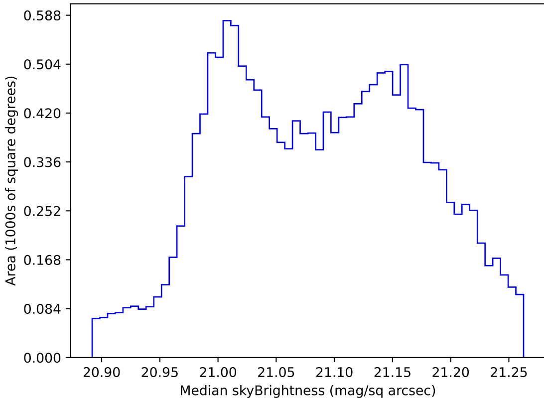
too_elab_r256_d2_ugrizy_v3.4_10yrs WFD r band: Median skyBrightness
