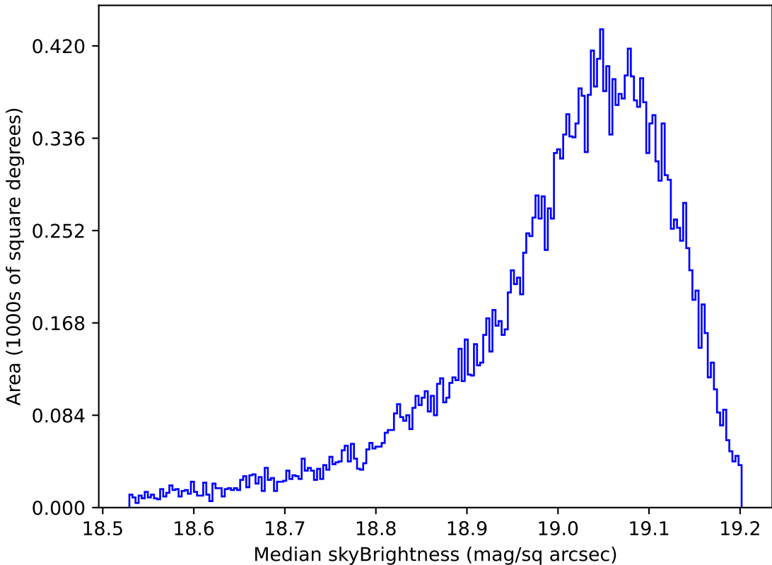
too_elab_r256_d2_ugrizy_v3.4_10yrs All sky z band: Median skyBrightness
