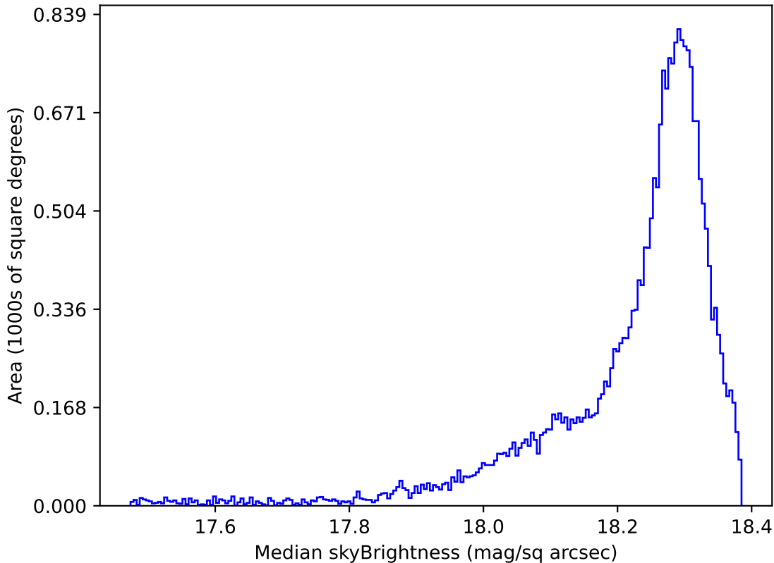
too_elab_r256_d2_ugrizy_v3.4_10yrs All sky y band: Median skyBrightness
