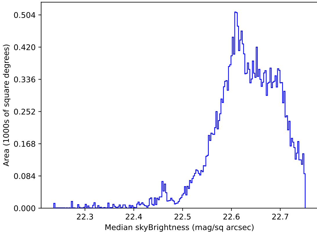
too_elab_r256_d2_ugrizy_v3.4_10yrs All sky u band: Median skyBrightness
