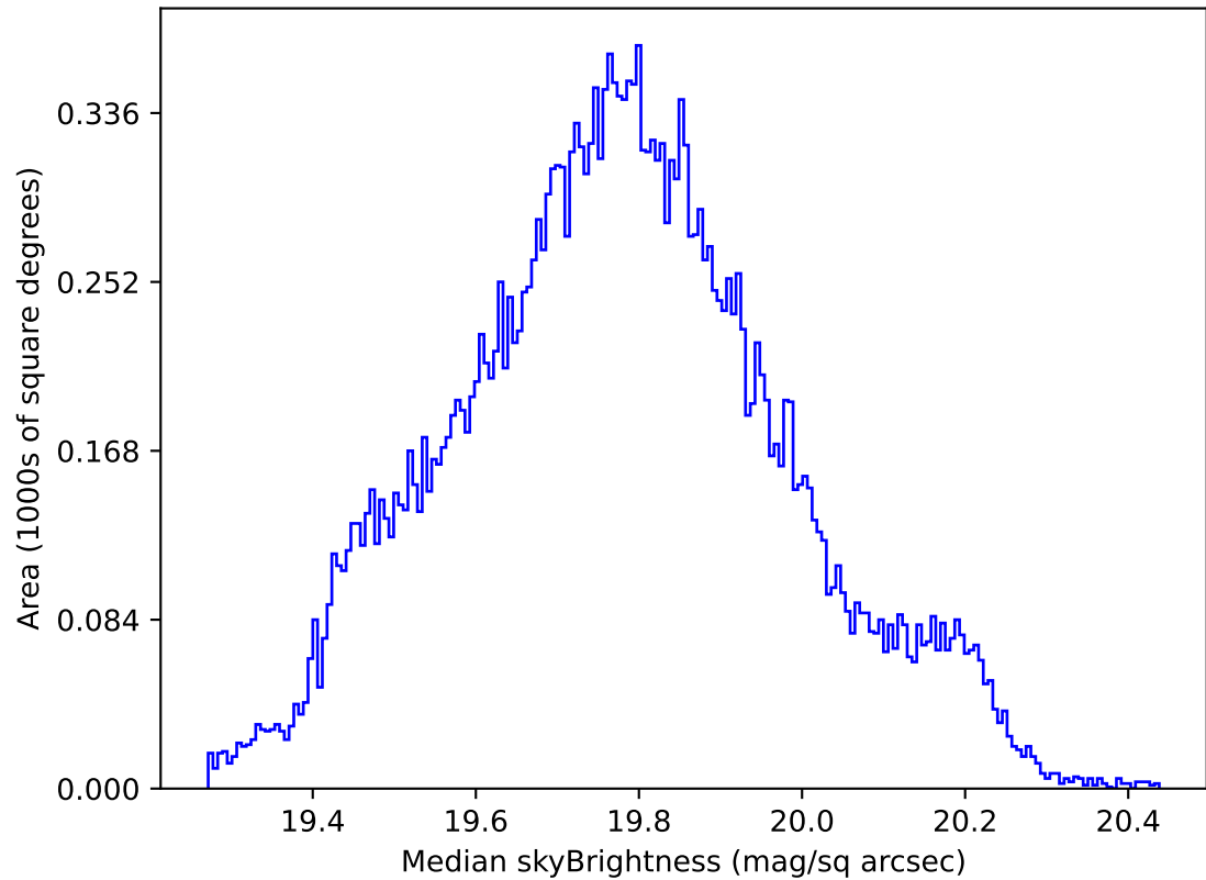
too_elab_r256_d2_ugrizy_v3.4_10yrs All sky all bands: Median skyBrightness
