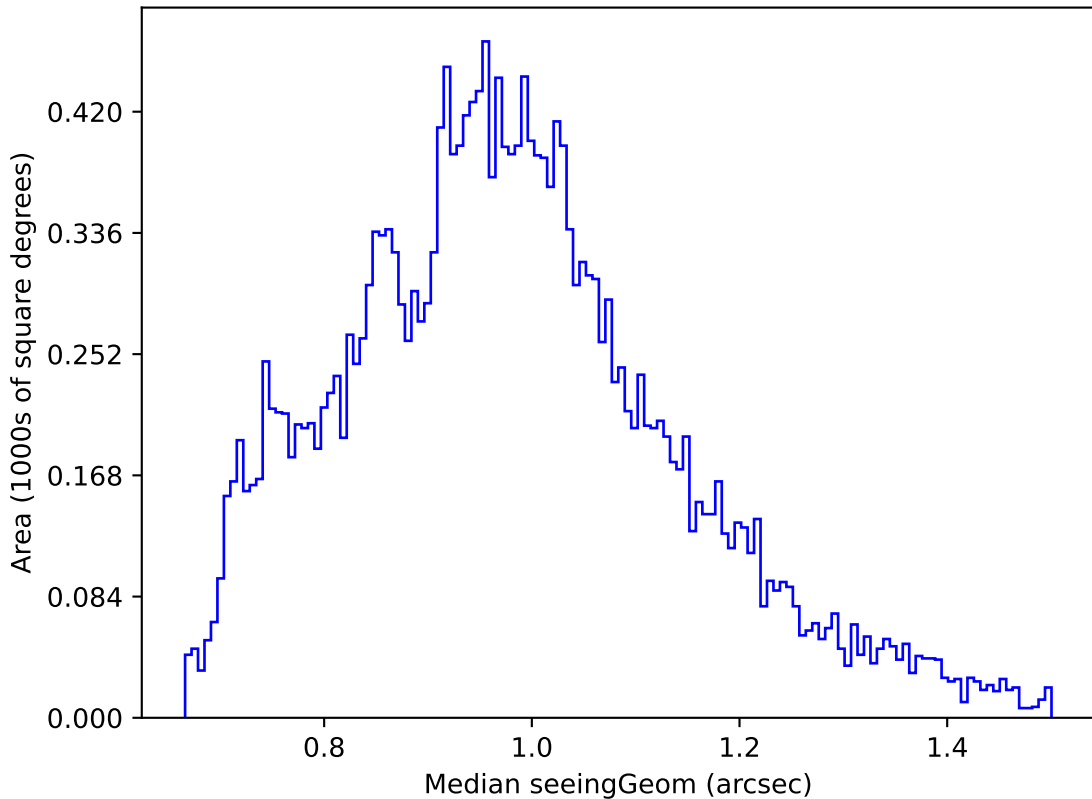
too_elab_r256_d2_ugrizy_v3.4_10yrs Yr 1 u band: Median seeingGeom
