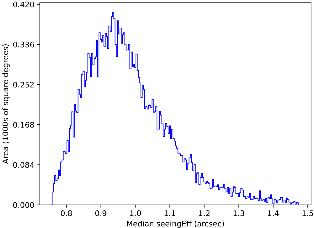
too_elab_r256_d2_ugrizy_v3.4_10yrs Yr 1 z band: Median seeingEff
