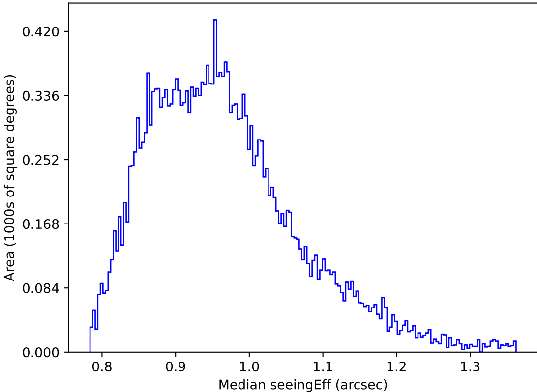
too_elab_r256_d2_ugrizy_v3.4_10yrs Yr 1 y band: Median seeingEff
