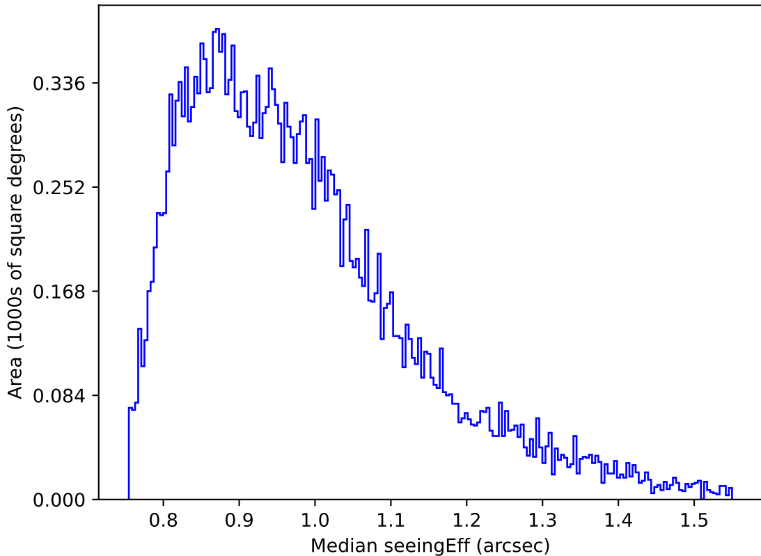
too_elab_r256_d2_ugrizy_v3.4_10yrs Yr 1 r band: Median seeingEff
