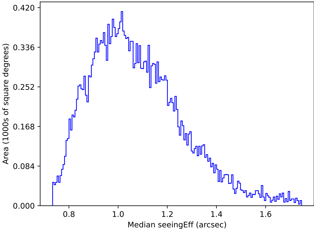
too_elab_r256_d2_ugrizy_v3.4_10yrs Yr 1 g band: Median seeingEff
