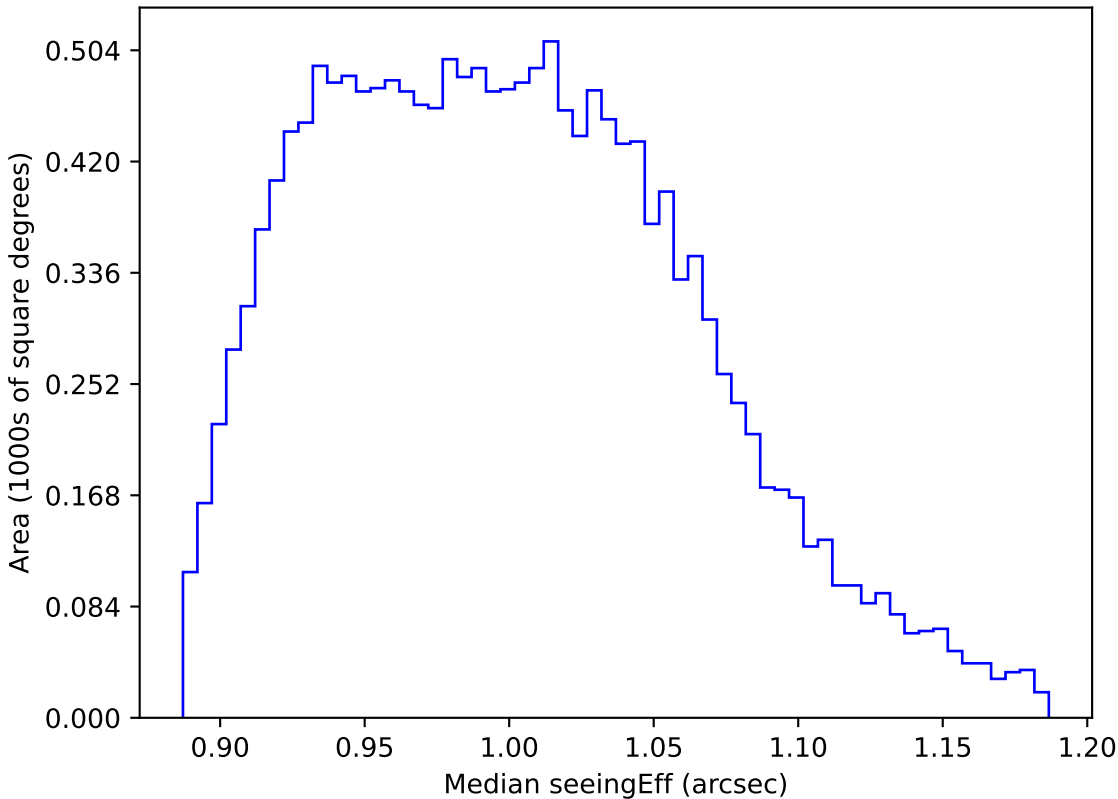
too_elab_r256_d2_ugrizy_v3.4_10yrs WFD y band: Median seeingEff
