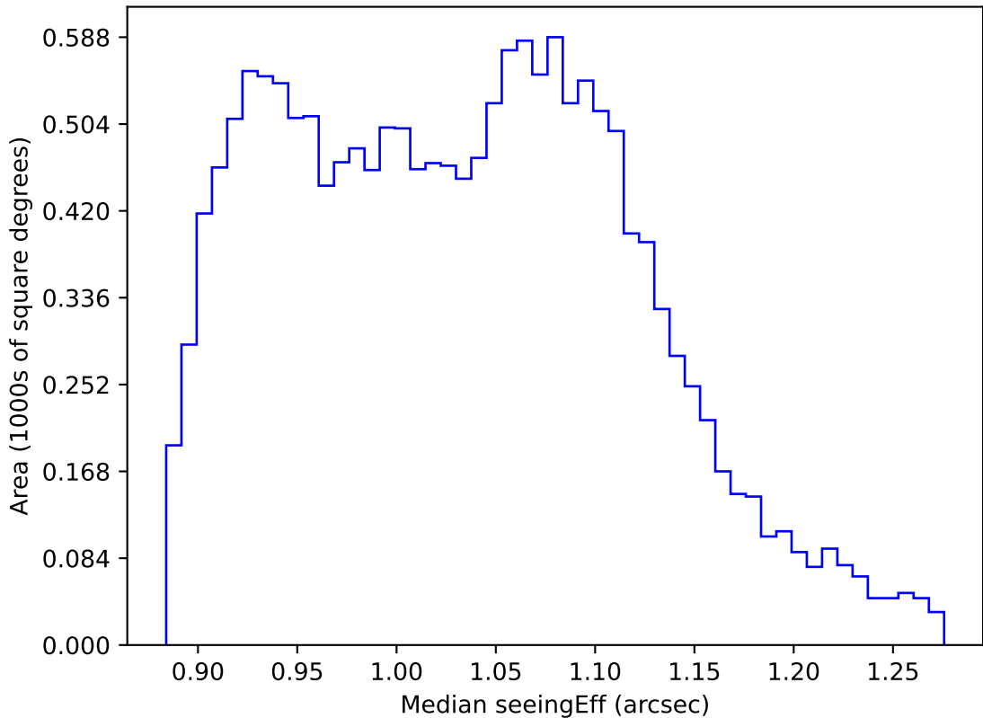
too_elab_r256_d2_ugrizy_v3.4_10yrs WFD r band: Median seeingEff
