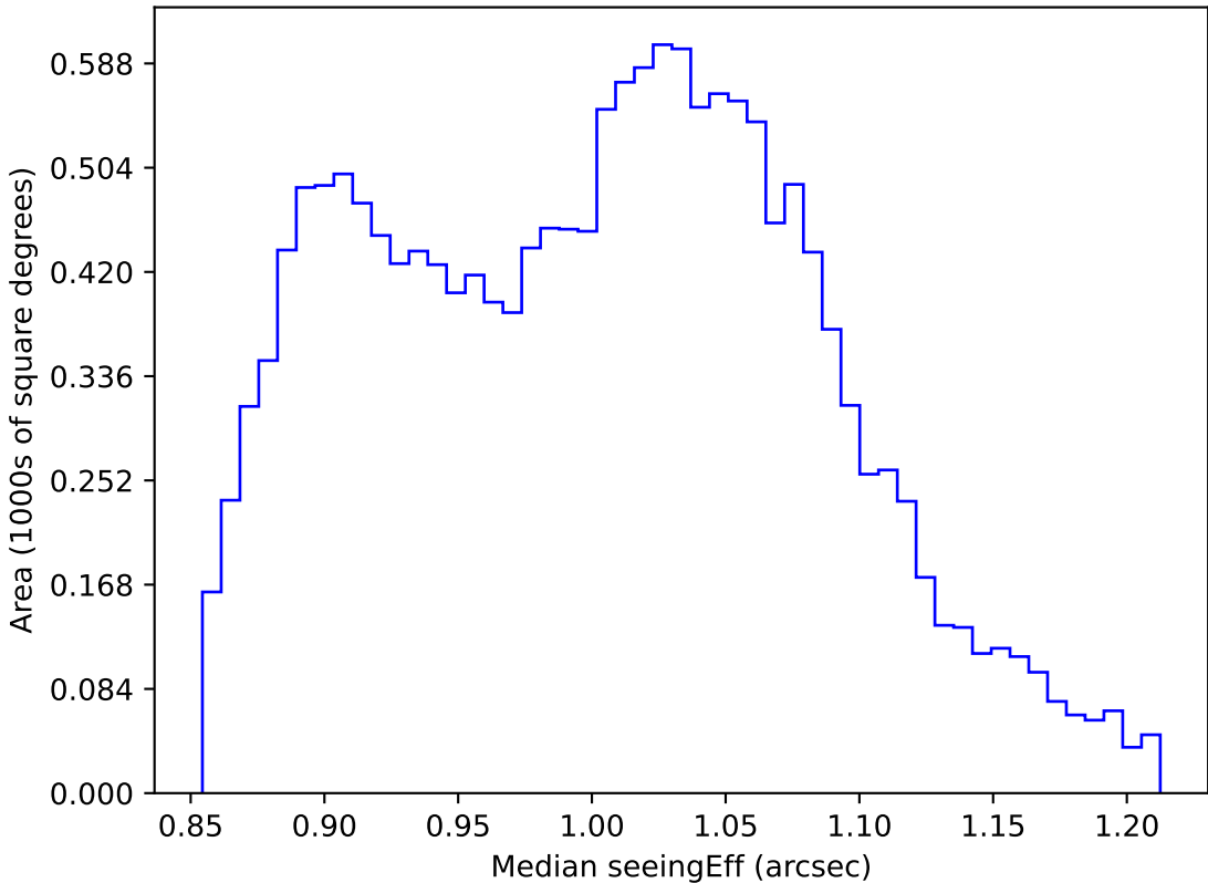
too_elab_r256_d2_ugrizy_v3.4_10yrs WFD i band: Median seeingEff
