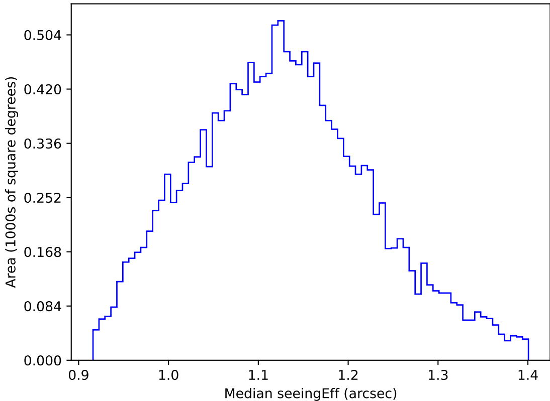
too_elab_r256_d2_ugrizy_v3.4_10yrs WFD g band: Median seeingEff
