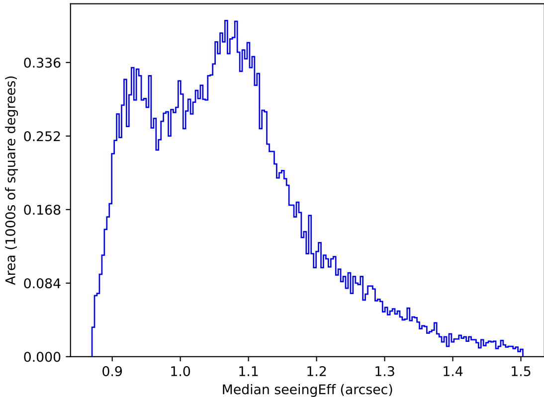
too_elab_r256_d2_ugrizy_v3.4_10yrs All sky r band: Median seeingEff
