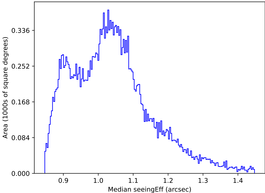
too_elab_r256_d2_ugrizy_v3.4_10yrs All sky i band: Median seeingEff
