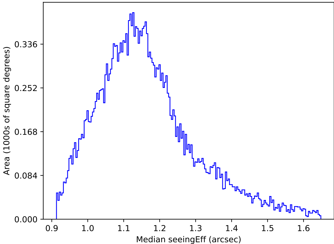
too_elab_r256_d2_ugrizy_v3.4_10yrs All sky g band: Median seeingEff
