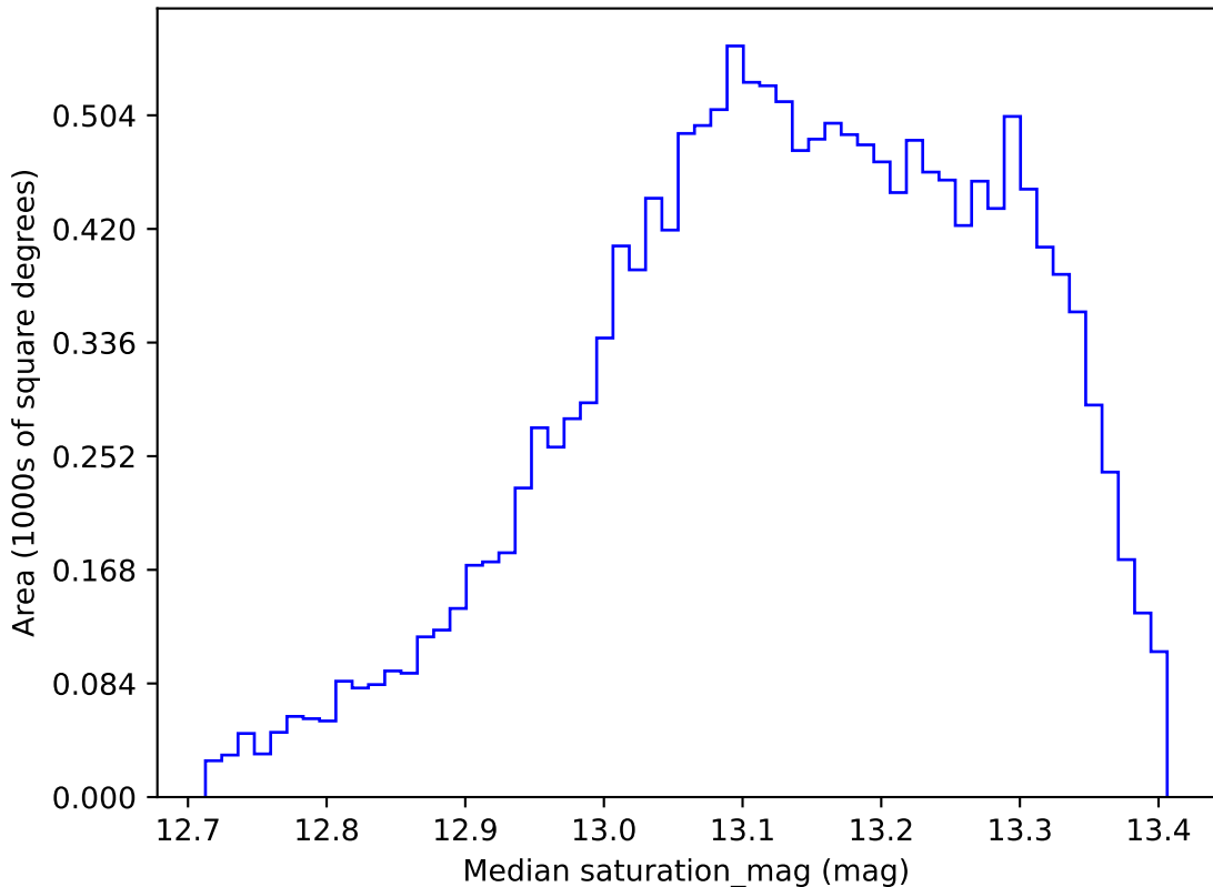
too_elab_r256_d2_ugrizy_v3.4_10yrs WFD y band: Median saturation_mag
