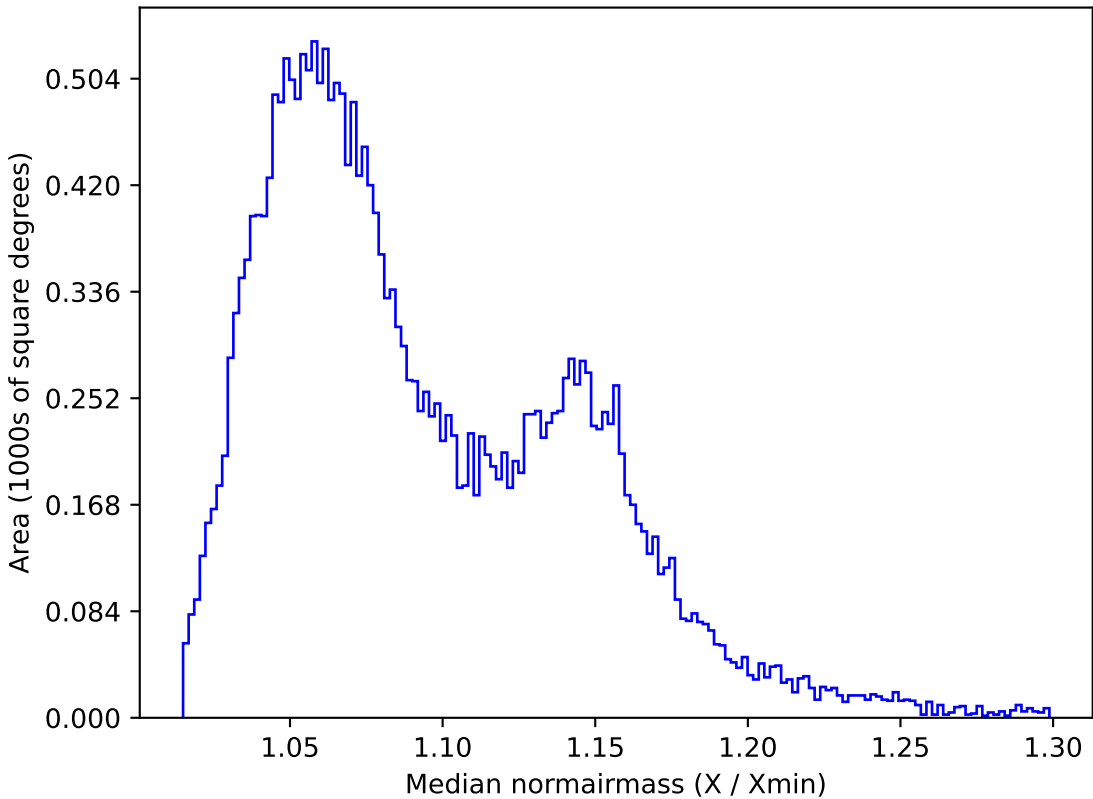
too_elab_r256_d2_ugrizy_v3.4_10yrs All sky y band: Median normairmass
