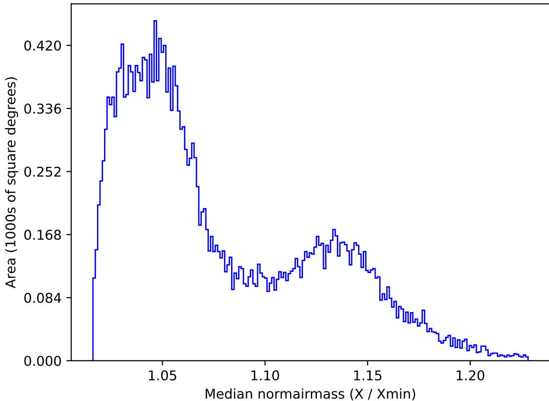
too_elab_r256_d2_ugrizy_v3.4_10yrs All sky r band: Median normairmass
