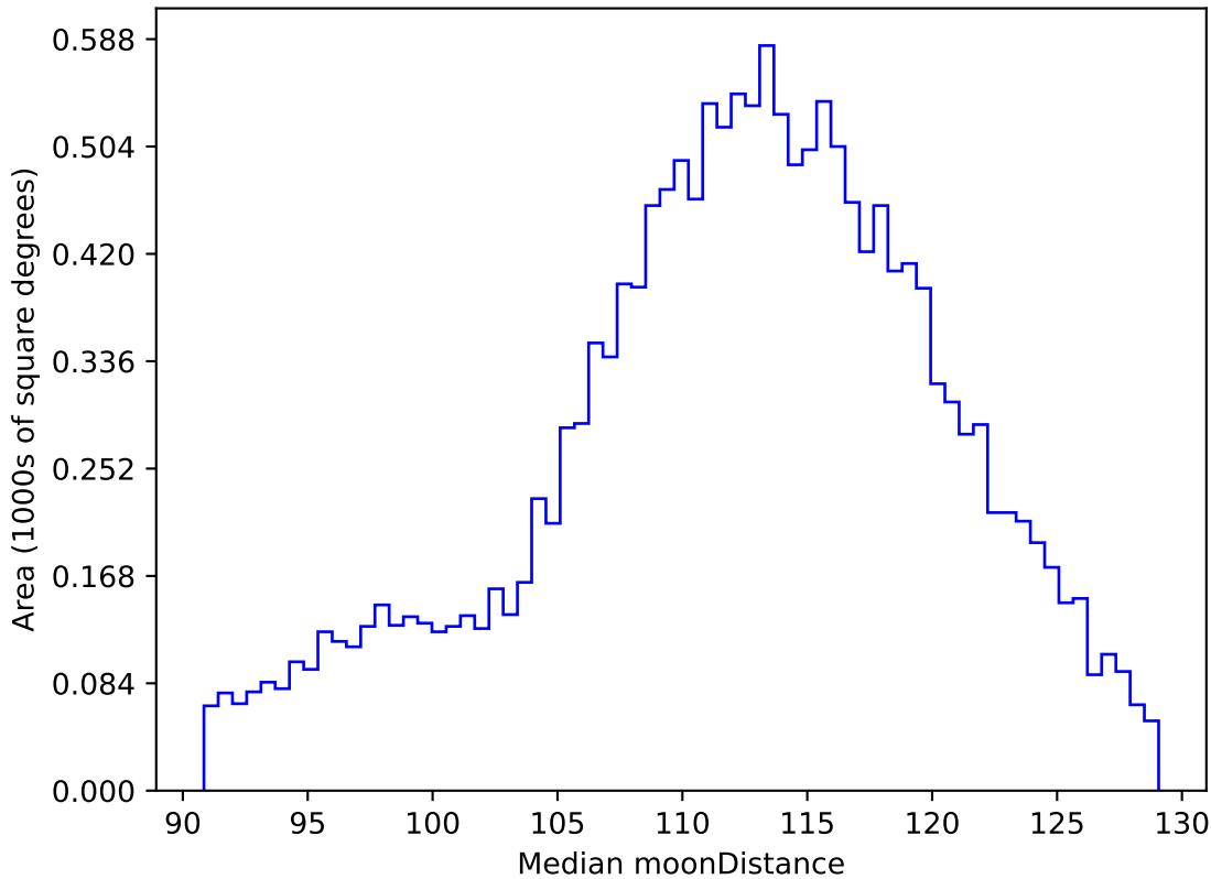
too_elab_r256_d2_ugrizy_v3.4_10yrs WFD r band: Median moonDistance
