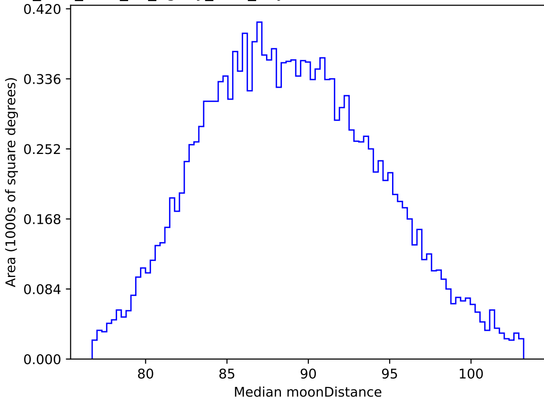
too_elab_r256_d2_ugrizy_v3.4_10yrs WFD all bands: Median moonDistance
