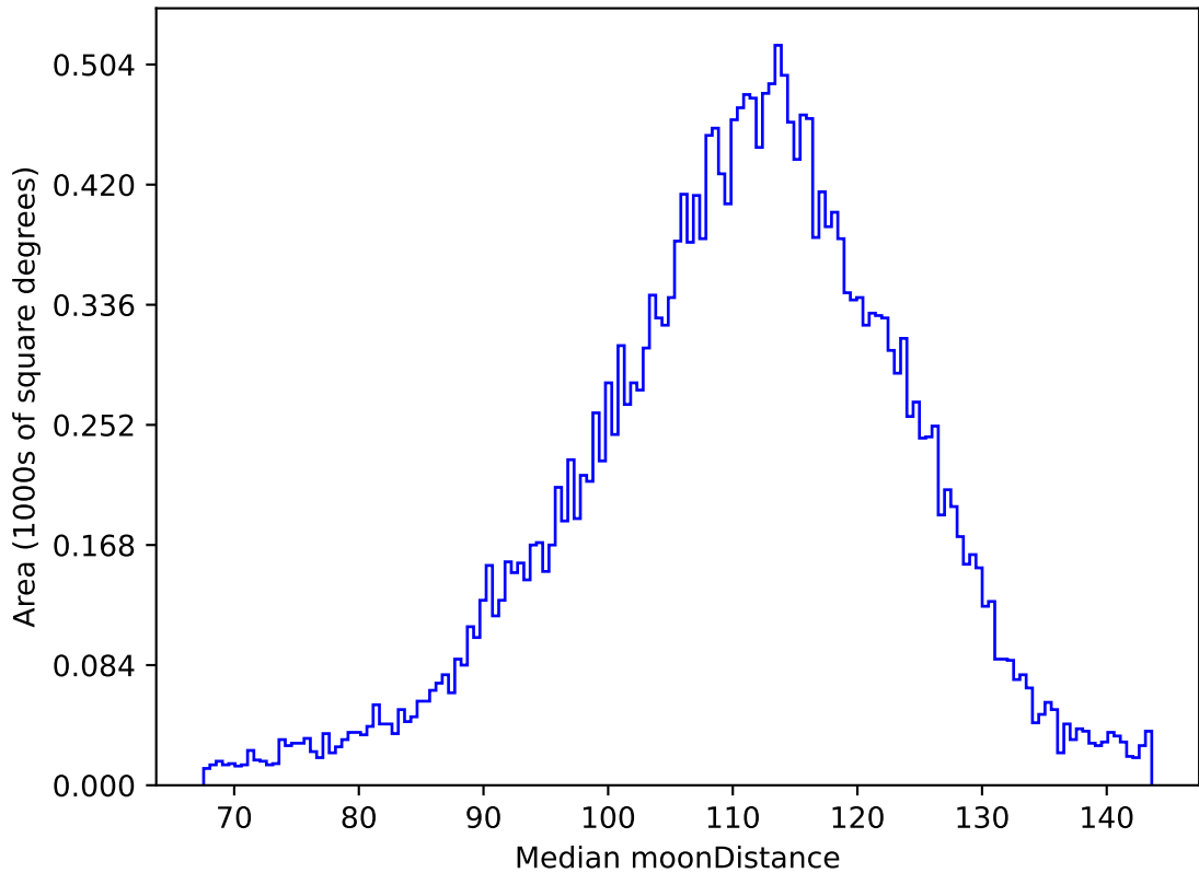
too_elab_r256_d2_ugrizy_v3.4_10yrs All sky g band: Median moonDistance
