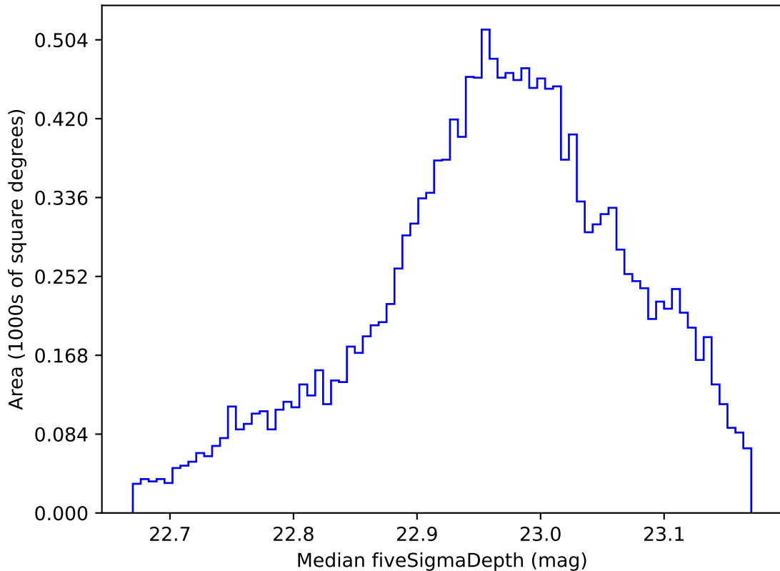
too_elab_r256_d2_ugrizy_v3.4_10yrs WFD z band: Median fiveSigmaDepth
